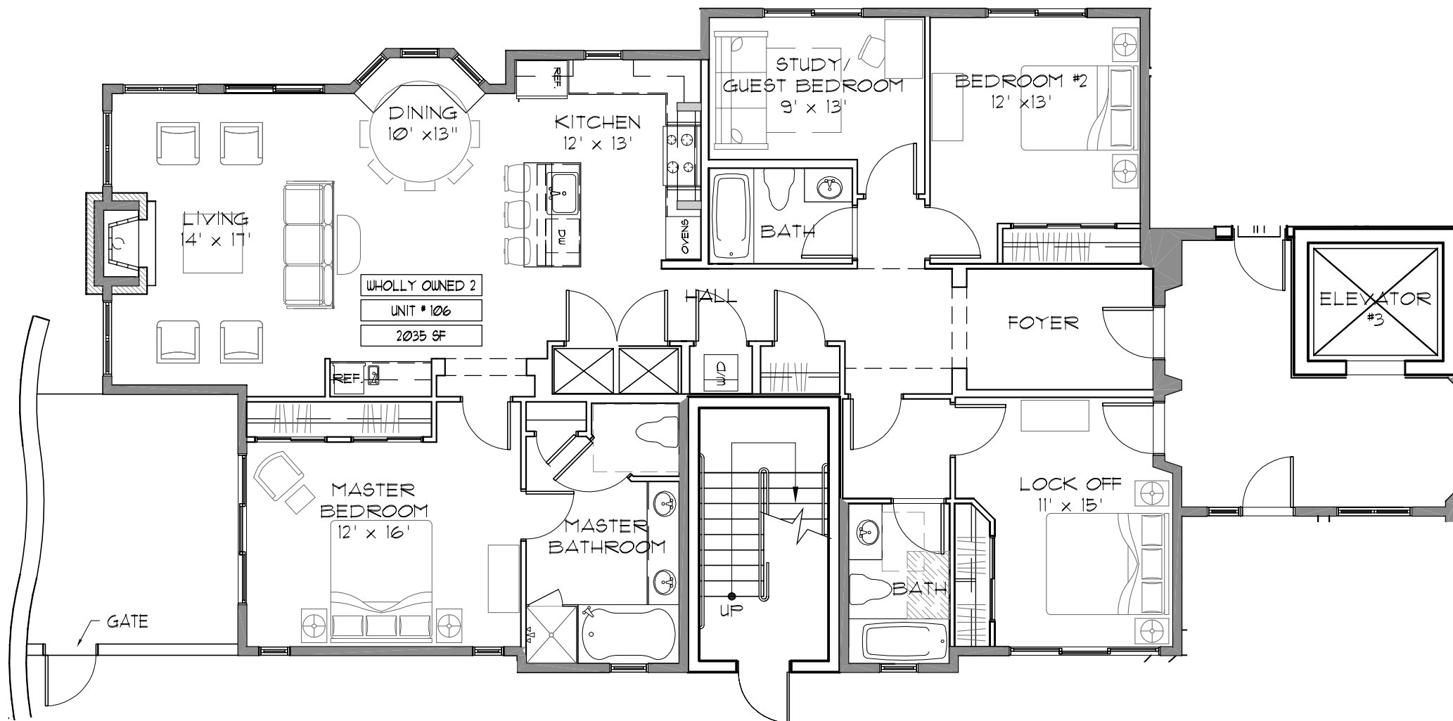
○ UNIT 105 1/8" = 1'-0"
